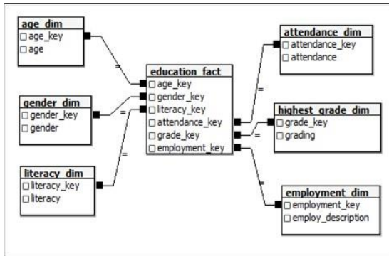
Fig. 2: Star Schema Design
